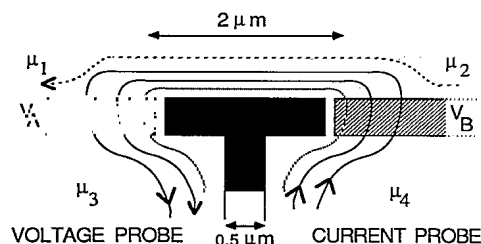
FIG. 3. Illustration of the selective population and detection of the first and second fractional edge channels. In this case the third channel does not contribute to the Hall conductance. The dotted line along the black center gate indicates the depletion area induced by the center gate voltage, which prevents conduction through the narrow openings separating the different gates.
