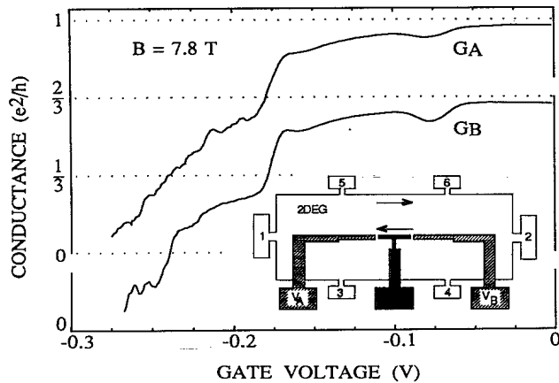
FIG. 1. Barrier conductances G_A and G_B as a function of gate voltage at a field of 7.8 T. The curve G_B has been offset for clarity. The double-barrier geometry defined by three different gates is shown in the inset. The arrows indicate the direction of electron flow along the sample edges.
