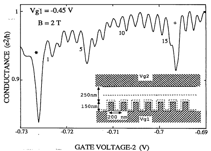
FIG. 2. Conductance as a function of gate voltage 2 V_{g2} on the second gate at 2 T and V_{g1} = -0.45 V on the first gate. The inset schematically shows the gate geometry; the dashed lines indicate the depletion regions in the 2DEG. The upper depletion region is moved towards the fingers when V_{g2} is made more negative.
