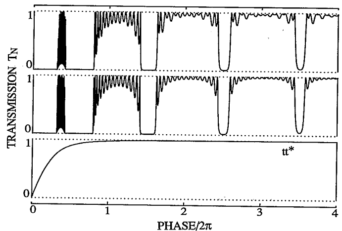
FIG. 3. Calculations from Eq. (1) of the transmission T_N as a function of phase \theta of a 1D chain of N=16 barriers. The lowest curve shows the simultaneously varying transmission probability t t^* through a single barrier. In the middle curve all barriers are taken equal, while in the upper curve a small amount of disorder is included by one deviating barrier.
