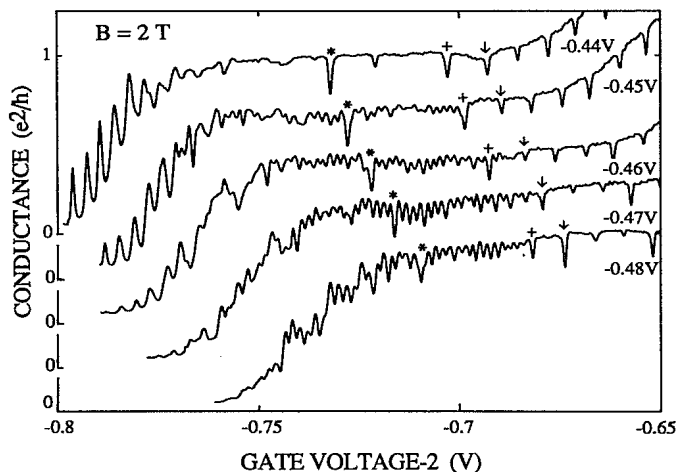
FIG. 1. Conductance as a function of gate voltage 2 V_{g2} on the second gate at a fixed magnetic field of 2 T and for different values of gate voltage 1 V_{g1} on the first gate. Corresponding peaks are marked. The curves have been offset for clarity.
